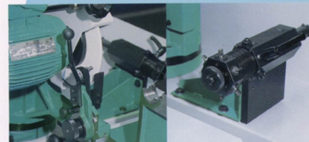
Quick adjusting multi-stylus arrangement (Visage Plus).
